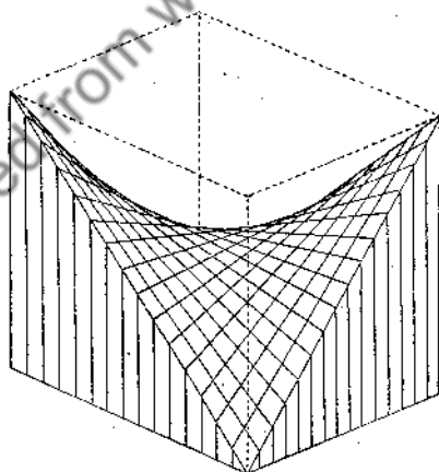
Fig. 39. Hyperbolic paraboloid
