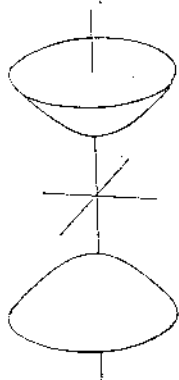
Fig. 23. Hyperboloid of two sheets.
