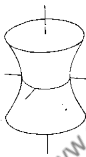
Fig. 24. Hyperboloid of one sheet.
