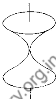
Fig. 26. Surface of revolution of parabola about vertical tangent
